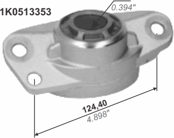
SOPORTE AMORTIGUADOR TRASERO (CAZOLETA) REAR SHOCK ABSORBER MOUNT
