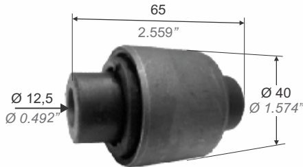
BUJE BIELETA TENSORA (LARGO) TENSILE BAR BUSHING (LONG)
